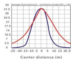
Average illumination curve
